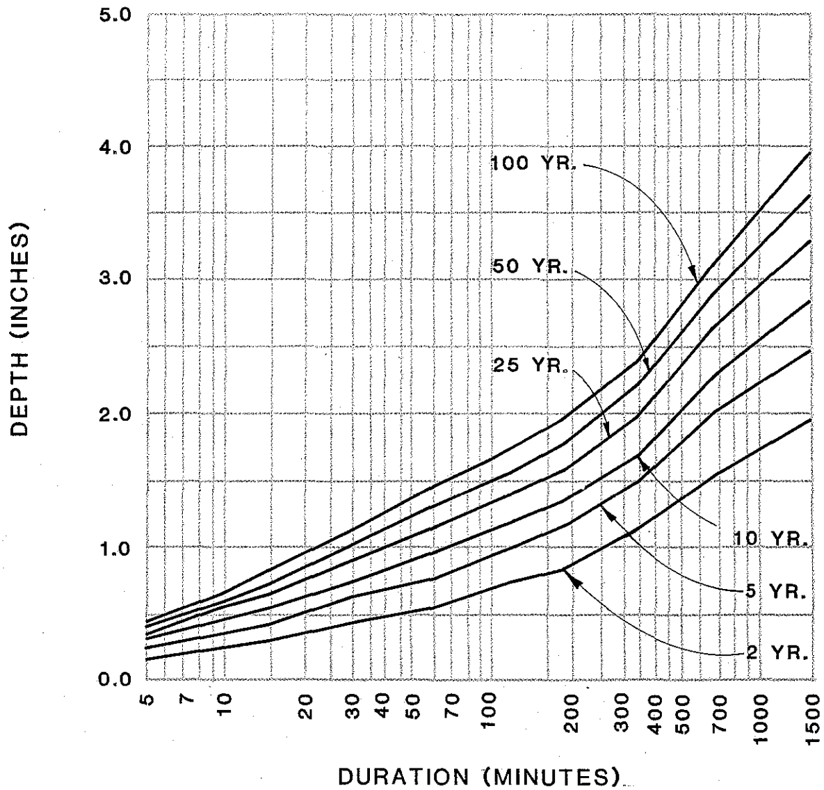
PROVO CITY STORM DRAINAGE MASTER PLAN RAINFALL DEPTH - DURATION - FREQUENCY CURVES FOR AREAS GREATER THAN 5000'
