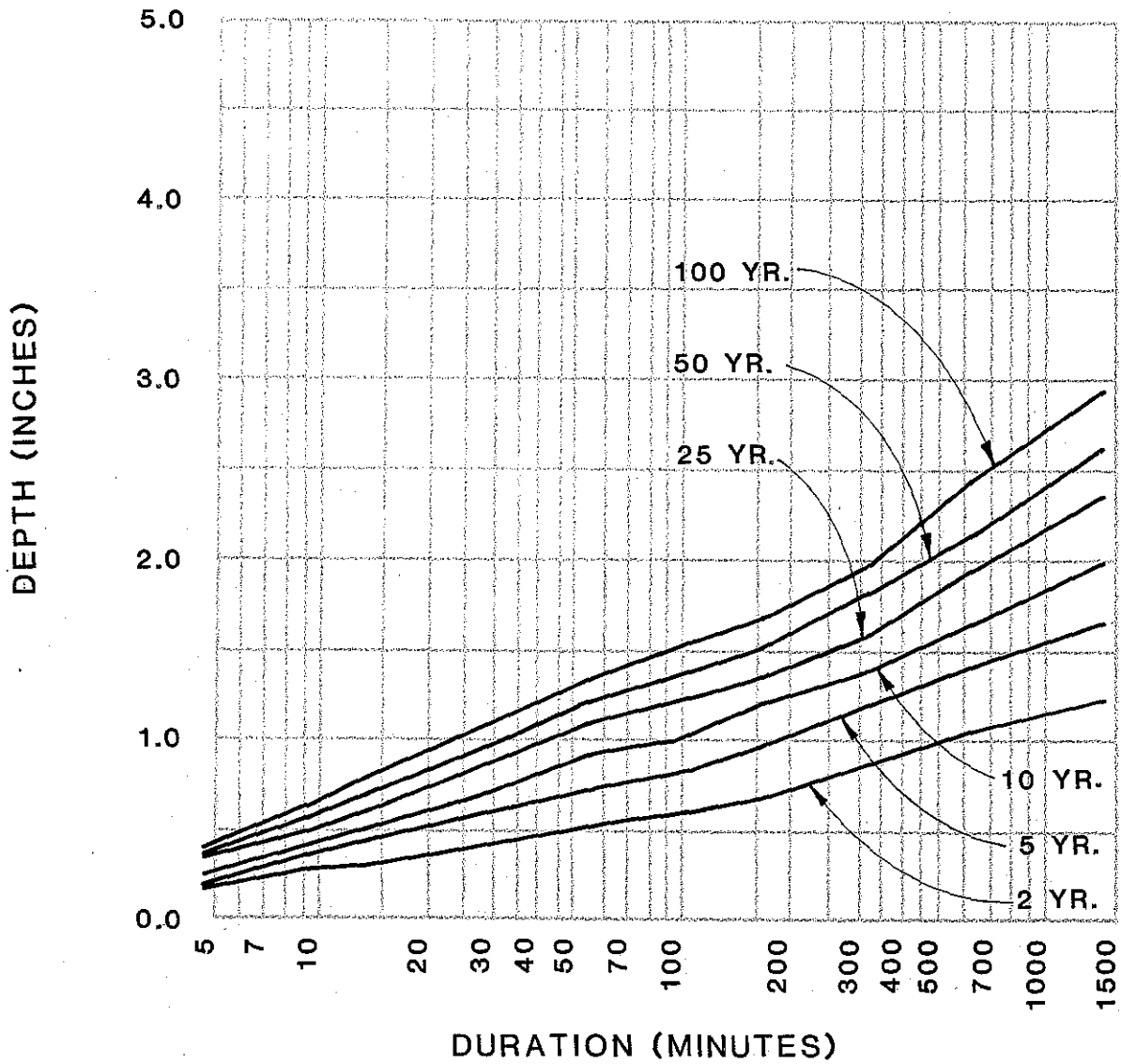
PROVO CITY STORM DRAINAGE MASTER PLAN RAINFALL DEPTH -DURATION- FREQUENCY CURVES FOR AREAS LESS THAN 5000'
